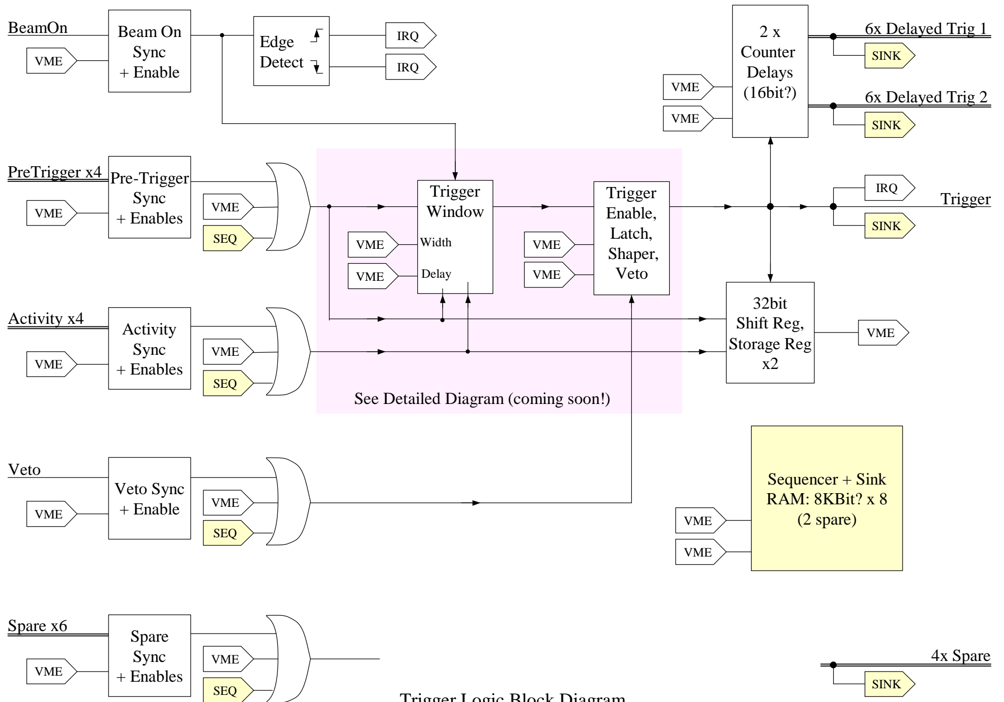
Trigger Logic Block Diagram
