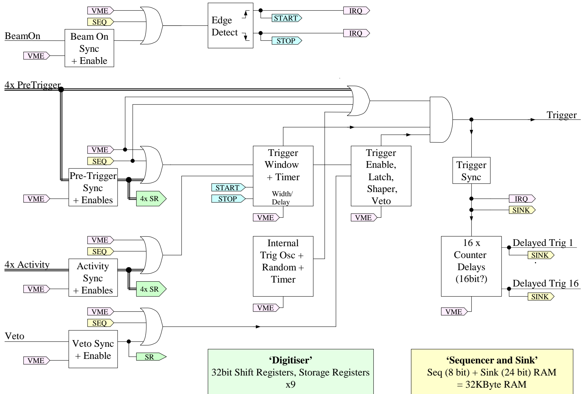
Trigger Logic Block Diagram
