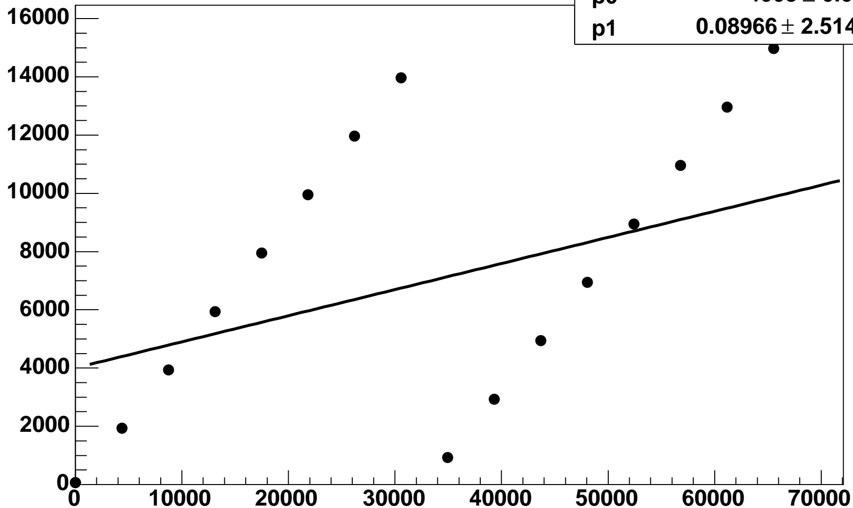
FE6, Chip 6, ADC mean vs DAC1
