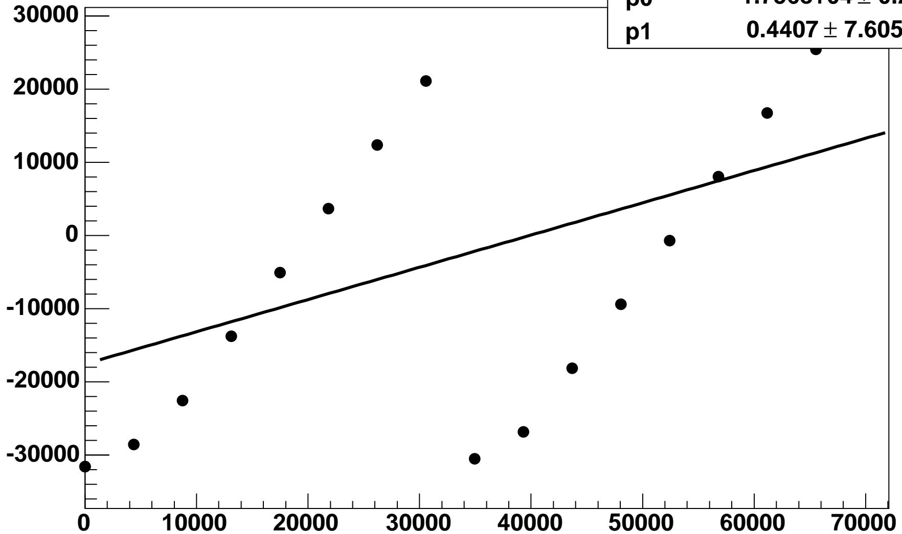
FE7, Chip 0, ADC mean vs DAC0
