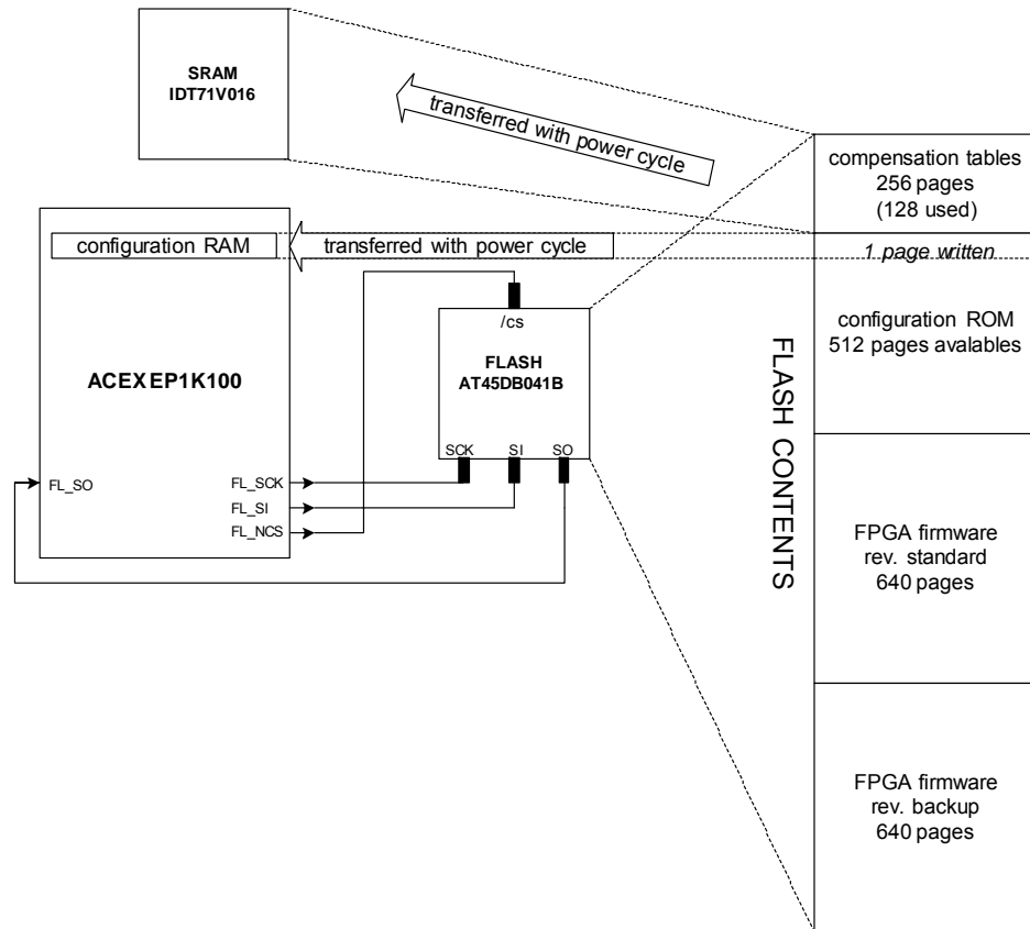
Fig. A.1: FLASH Architecture (V1290 A)
