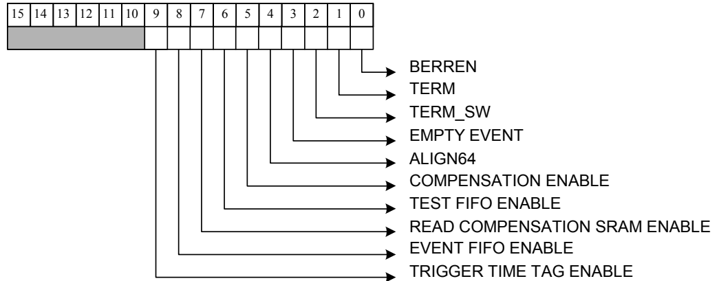
Fig. 6.9: Control Register
