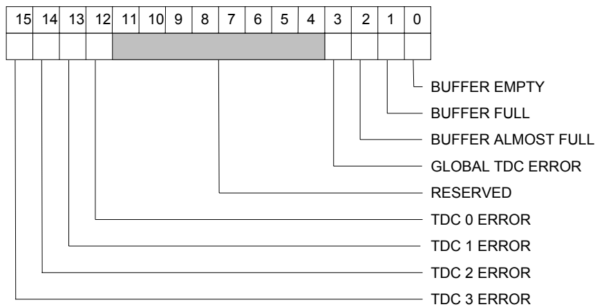
Fig. 3.15: Status Register 2
