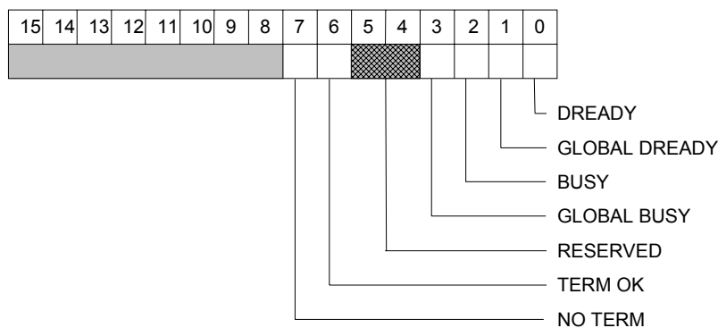
Fig. 3.9: Status Register 1
