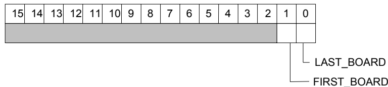
Fig. 3.14: Control Register 1
