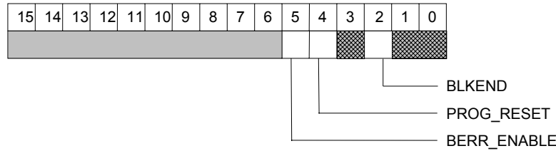
Fig. 3.10: Control Register 1
