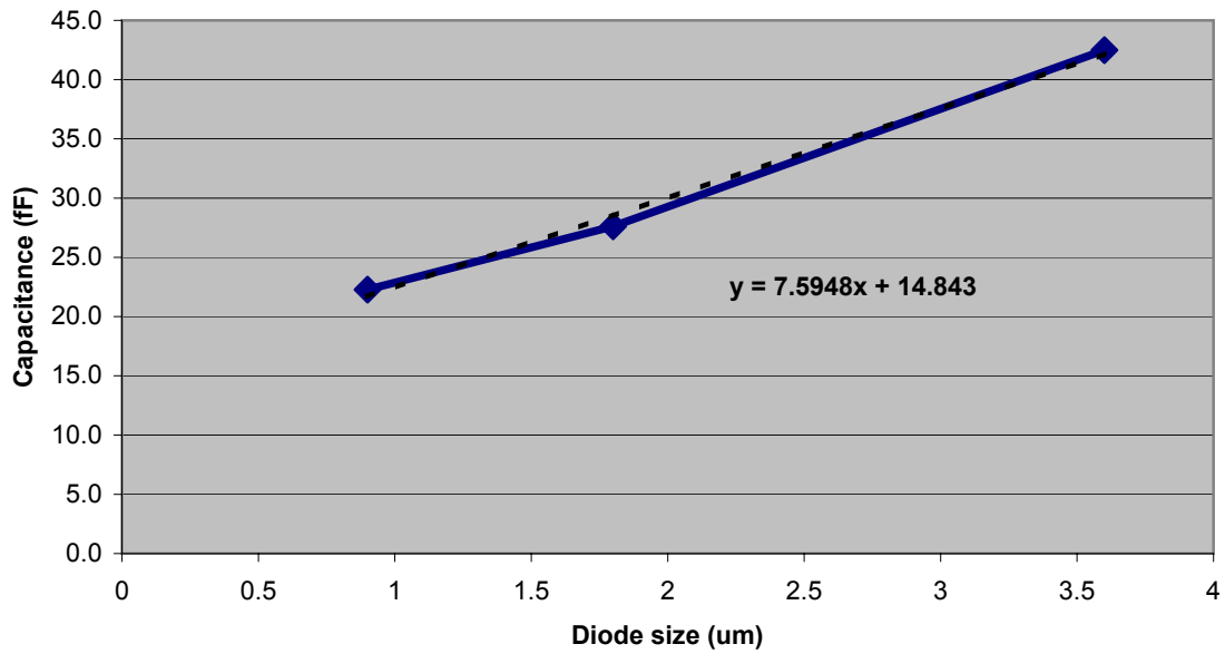
Capacitance at DIODENODE (extracted view)
