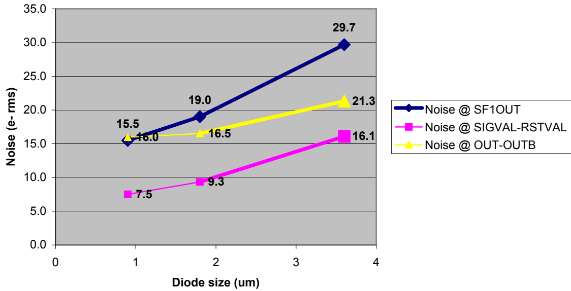
Noise in Presample (extracted view)
