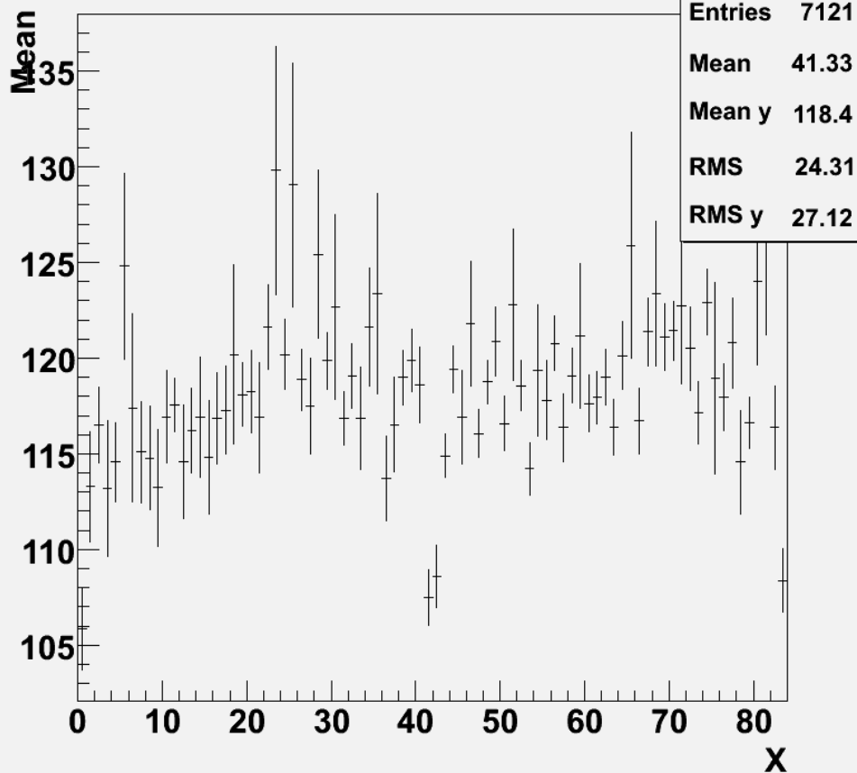
Row Fe55 Means with ped Quad0
