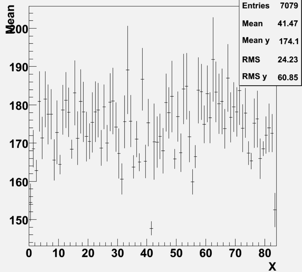
Row Fe55 Means with ped Quad1
