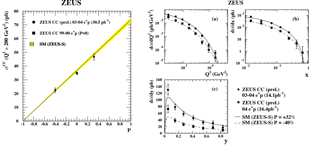
FIGURE 1. The total cross section for e^+p CC DIS as a function of the longitudinal polarisation of the positron beam is shown on the left. On the right the differential cross-sections (a) d\sigma/dQ^2 , (b) d\sigma/dx and (c) d\sigma/dy are shown. The curves show the SM predictions evaluated using the ZEUS-S PDFs.
