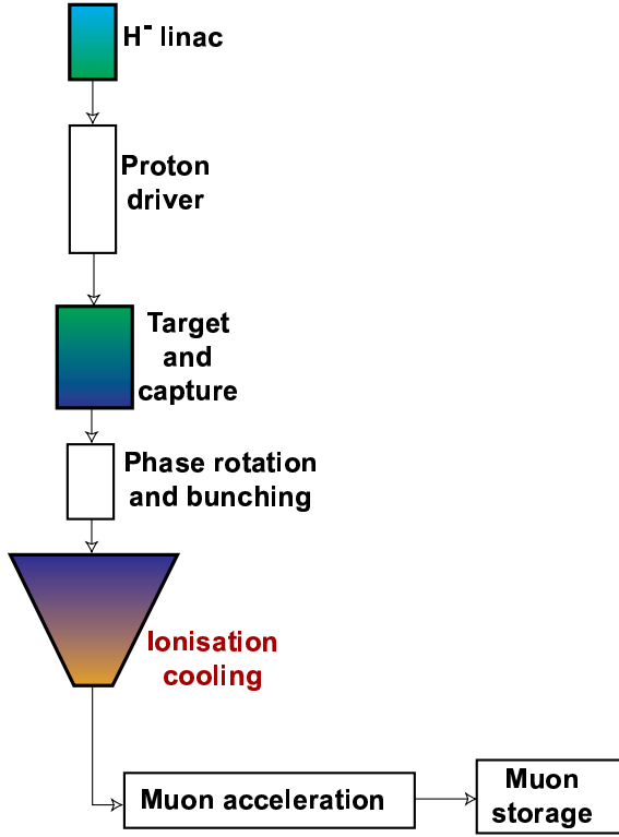
Figure 1. Schematic drawing showing the major sub-systems in the Neutrino Factory accelerator complex.
