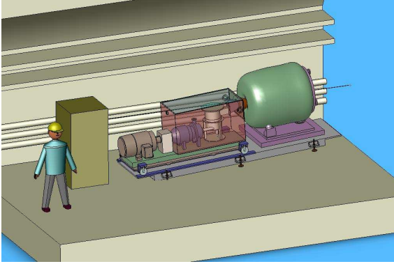
Figure 2. Schematic diagram of the MERIT experiment at the neutron time-of-flight (nToF) facility at CERN [47].
