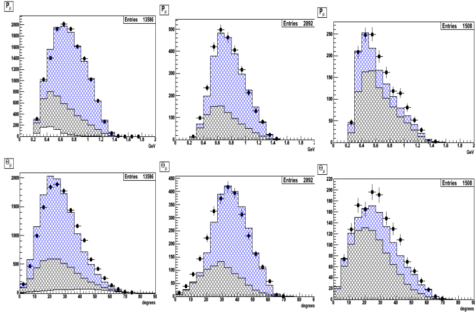
Fig. 5. SciBooNE CC QE data: muon momentum (top) and angles (bottom) for SciBar-MRD matched sample. The left panels show one-track events, the centre panels show two track \mu-p events and the right panels show two-track \mu-\pi events. The data (points) include statistical uncertainties only. The MC (histogram) is split into three components: CC QE (blue), non-QE (black) and events originating outside the SciBar fiducial volume (white). The MC was generated with M_A^{\text{QE}}=1.21 \text{ GeV}/c^2 and is normalised to the MRD-matched data.[31]
