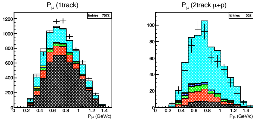
Fig. 13. SciBooNE antineutrino right-sign (left) and wrong-sign (right) muon momentum distributions. The data (black points) are shown with statistical uncertainties and MC wrong-sign (cyan) and right-sign (all other colours) contributions are indicated. [47].
