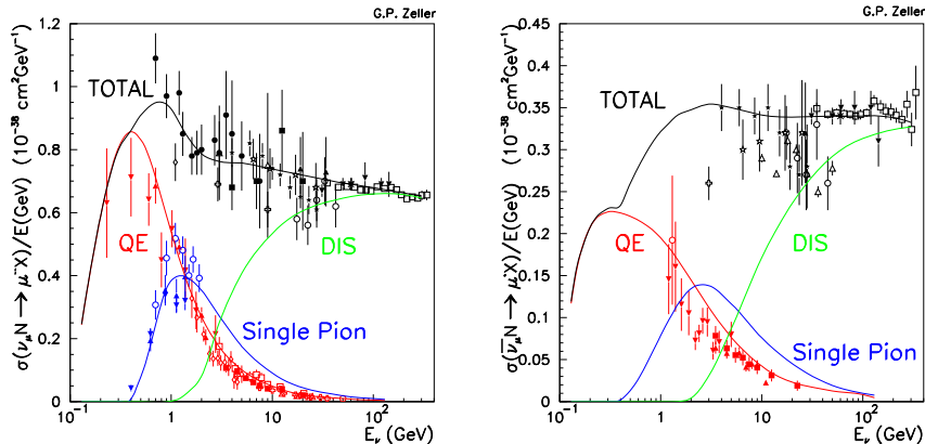
Fig. 1. Past measurements of neutrino (left) and antineutrino (right) cross sections. [2]
