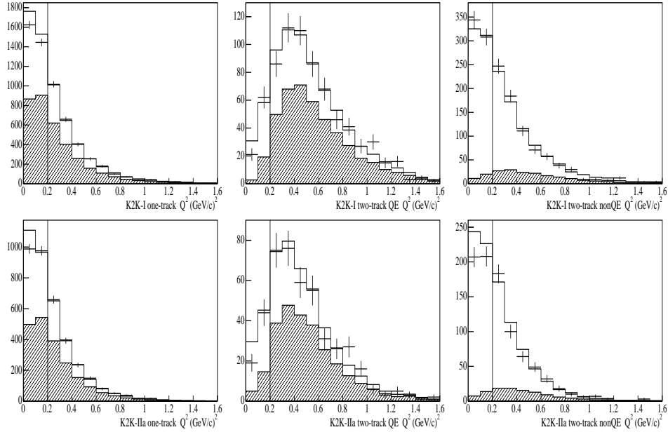
Fig. 3. K2K SciFi CC QE data: reconstructed Q^2 distributions for K2K-1 data (top) and K2K-IIa data (bottom) for the 1-track, 2-track QE enhanced, and 2-track non-QE enhanced samples. The shaded region shows the QE fraction of each sample, estimated from the MC. The lowest two data points in each plot are not included in the fit. [24]
