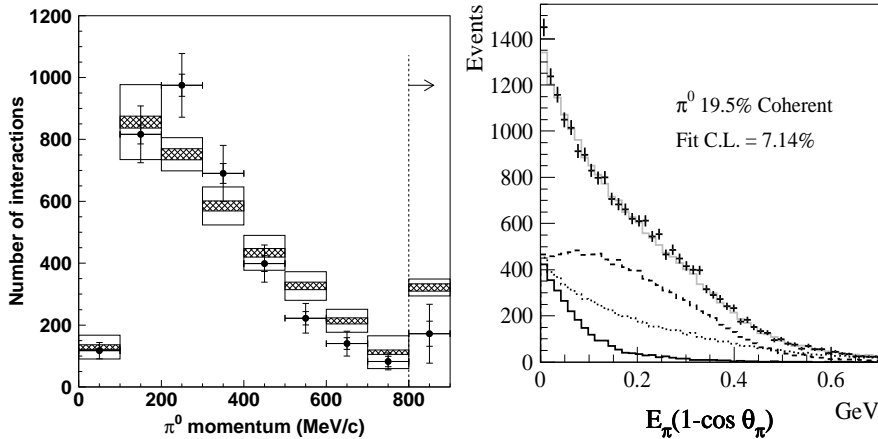
Fig. 10. K2K and MiniBooNE NC 1\pi^0 data. Left: momentum distribution of K2K NC 1\pi^0 data (black dots). The inner and outer error bars attached to data points show statistical errors and total errors including systematic errors, respectively. The MC simulation is also shown as a box histogram; the inner boxes represent MC statistical errors and the outer boxes represent the cross section model uncertainty. Right: energy weighted angular distribution of MiniBooNE data (crosses) and the histograms showing the coherent (solid), resonant (dashed) and background (dotted) contributions as predicted by MC after fitting to the data [41, 42].
