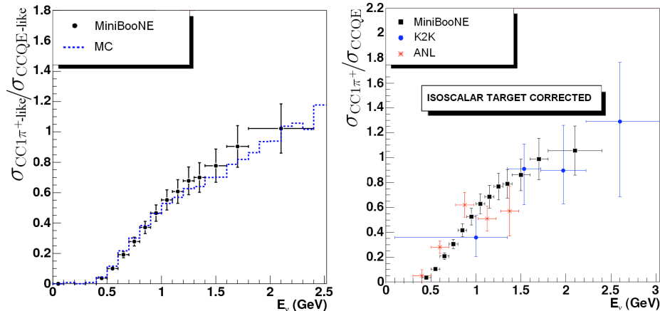
Fig. 8. MiniBooNE CC 1\pi^+ /CC QE ratio measurement (left) and comparison of MiniBooNE data with results from K2K and ANL.[38]
