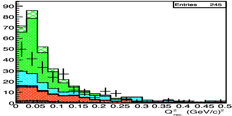
Fig. 14. SciBooNE antineutrino coherent pion sample reconstructed Q^2 distribution. Data (black crosses) are shown with statistical uncertainty, as well as MC CC coherent pion (green), wrong-sign (cyan), \bar{\nu}_\mu CC QE (red) and \bar{\nu}_\mu CC 1\pi^+ (incoherent) contributions from the MC. [47].
