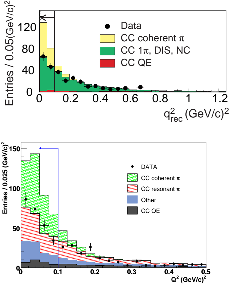
Fig. 9. K2K and SciBooNE neutrino coherent pion search data. Each plot shows reconstructed Q^2 distributions for the coherent pion enhanced samples, which are \mu-\pi non-QE events with low vertex activity. The top panel shows K2K SciBar data and best fit MC [39], and the bottom panel shows SciBooNE data with best fit MC [40].
