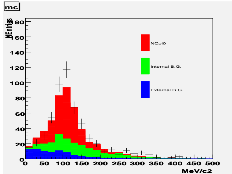
Fig. 11. SciBooNE's reconstructed invariant mass for \nu_\mu NC 1\pi^0 candidates contained within SciBar [43]. Data (crosses) are shown with statistical errors as well as signal NC 1\pi^0 (red), internal background (green) and external background (blue) contributions predicted by the MC simulation.
